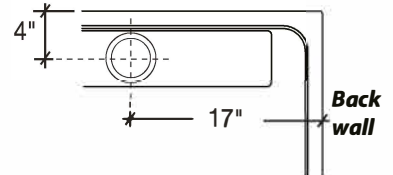
Drain Location Detail
